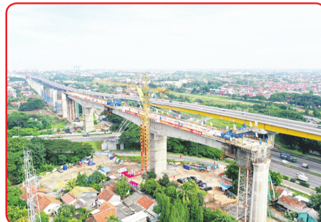
Continuous Beam DK20 + 156 Kereta Cepat Jakarta Bandung.
